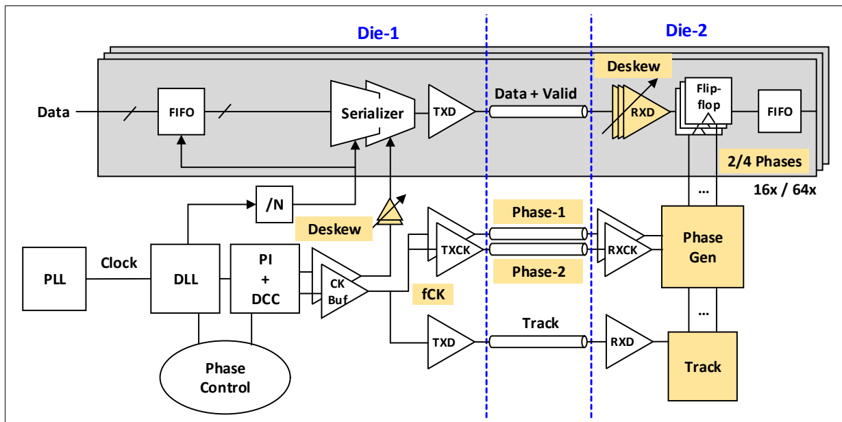
Figure 5-13. Clocking architecture
