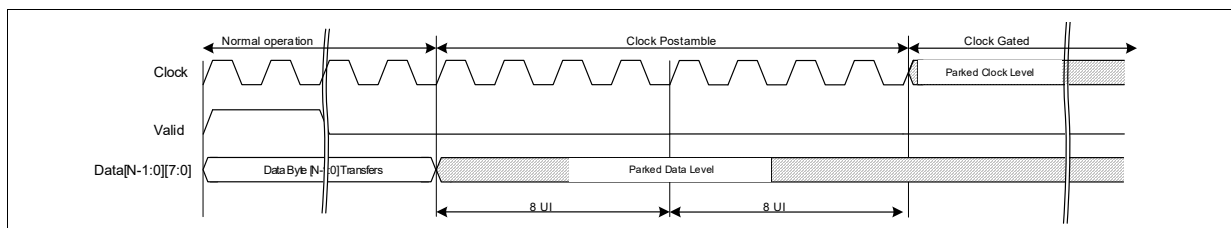
Figure 4-7. Clock gating
