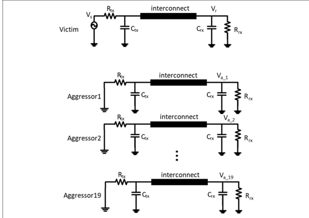
Figure 5-17. Circuit for VTF calculation
