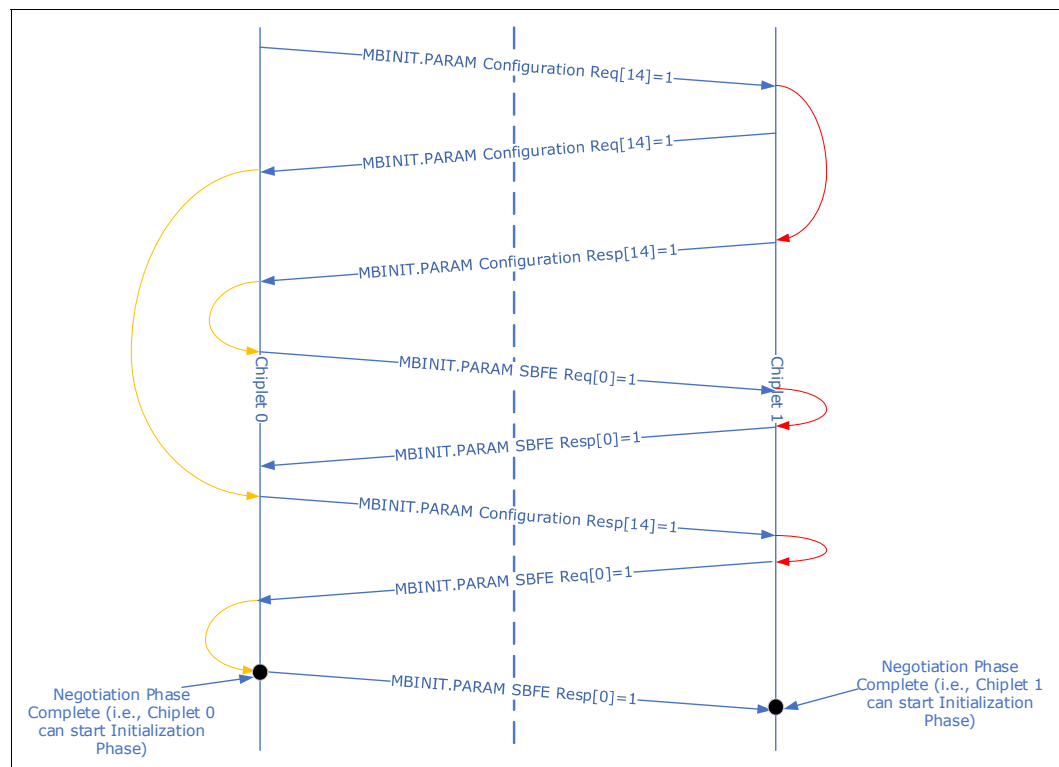
Figure 4-35. Example Sideband Management Transport Protocol Negotiation – Single-module Scenario
