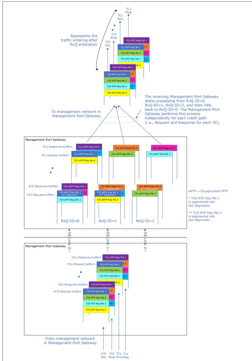
Figure 8-42. Conceptual Illustration of Sideband Multi-module Ordering with Three RxQs
