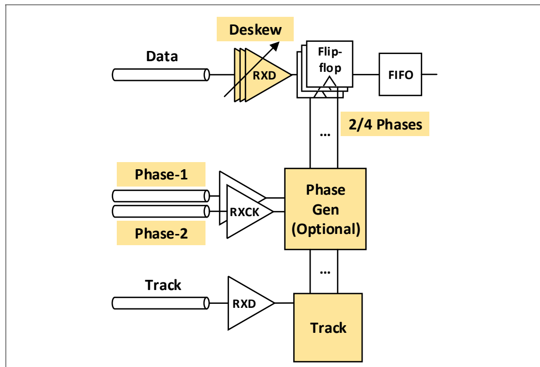
Figure 5-8. Receiver topology
